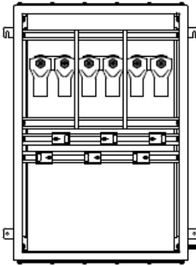
HVJB X3 (0-2) Cables entering from bottom only
